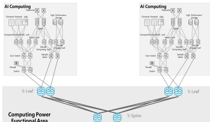
Figure 3-3 Computing power-oriented POP Zone
